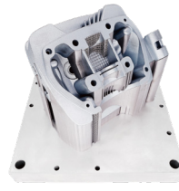
缸头 铝合金 190mm*140mm*155mm
